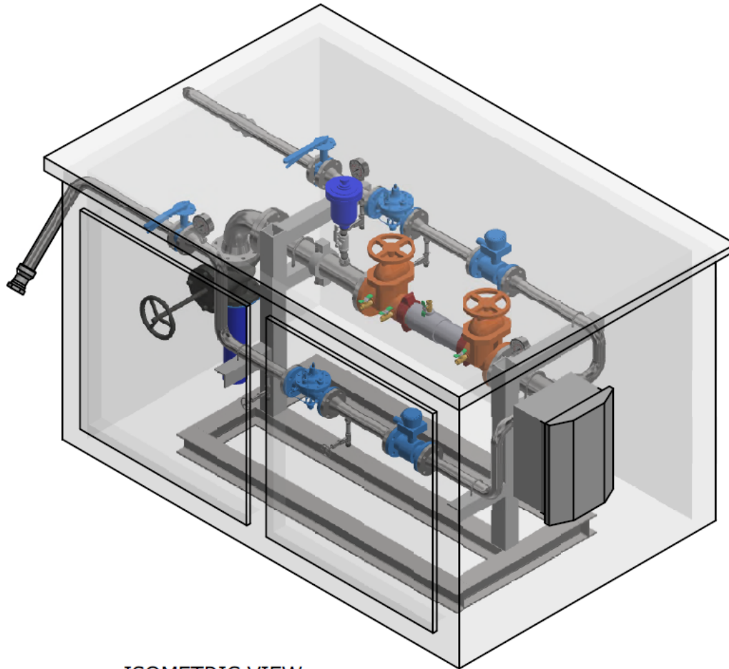
ISOMETRIC VIEW
